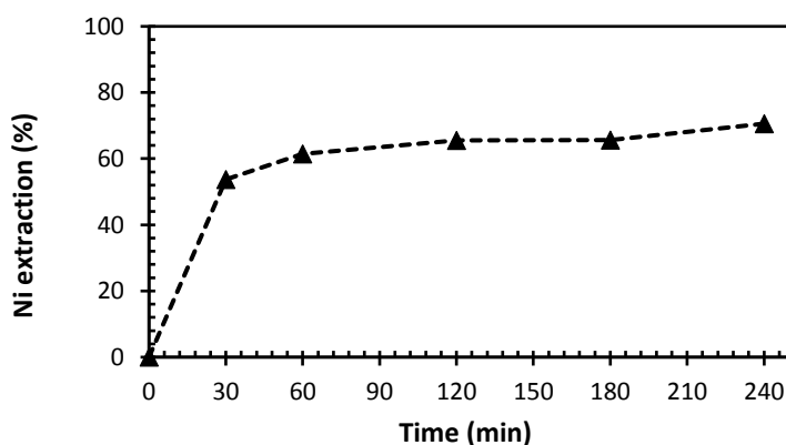
Fig. 7. The effect of the contact time on Ni extraction; operation conditions: 5 M H 2 SO 4 , 90 °C, 0.25 g/cm 3 , 300 rpm
