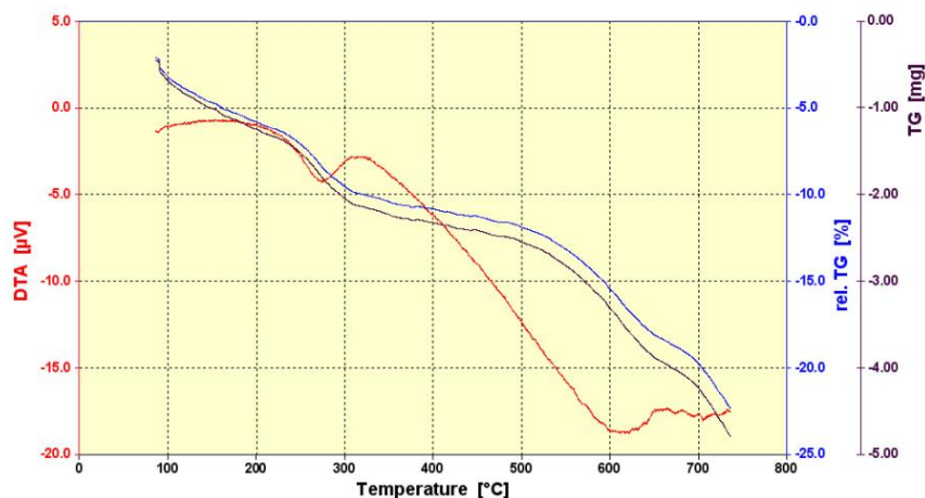
Fig. 8. TG/DTA curve for Sarbisheh nickel laterite ore
