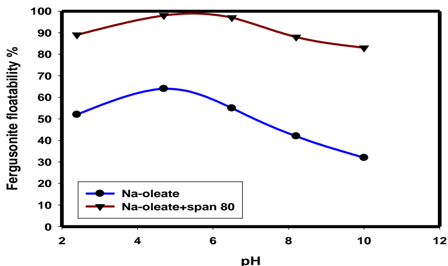
Fig. 5. Effect of pH on floatability of fergusonite using Na-oleate and the mixture collectors
