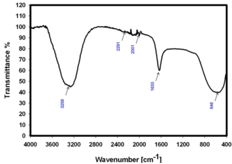
Fig. 8. FT-IR spectra of collector mixture
