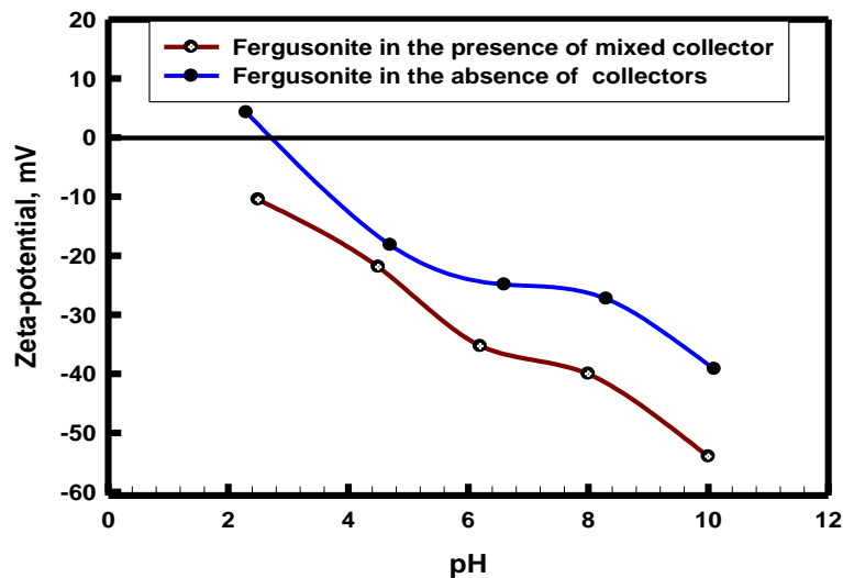
Fig. 7. Effect of mixture of sodium oleate and span 80 on zeta-potential of fergusonite
