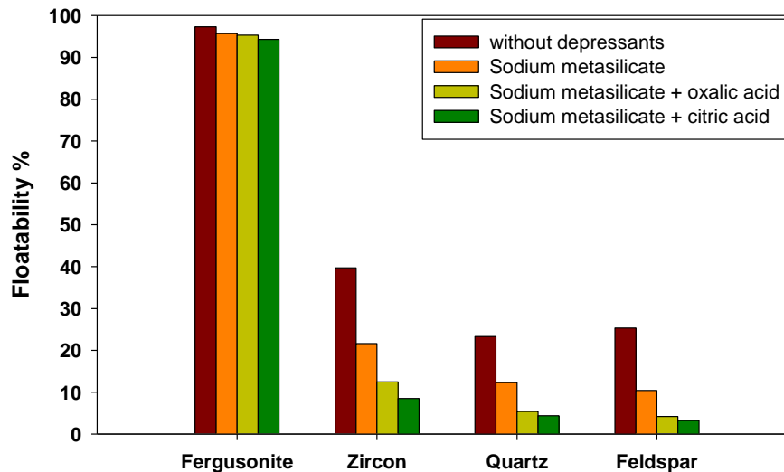
Fig. 6. Effect of addition of depressants on floatability of fergusonite and associated gangue minerals (zircon, quartz, and feldspar)
