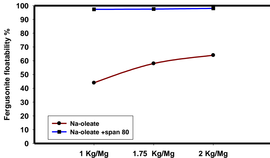
Fig. 4. Effect of collector dosage on floatability of fergusonite using sodium oleate and mixture of sodium oleate and span 80
