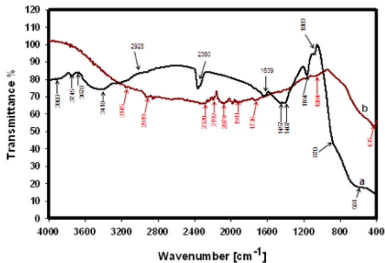
Fig. 9. FT-IR spectra of fergusonite (a), fergusonite treated with mixed collector (b)
