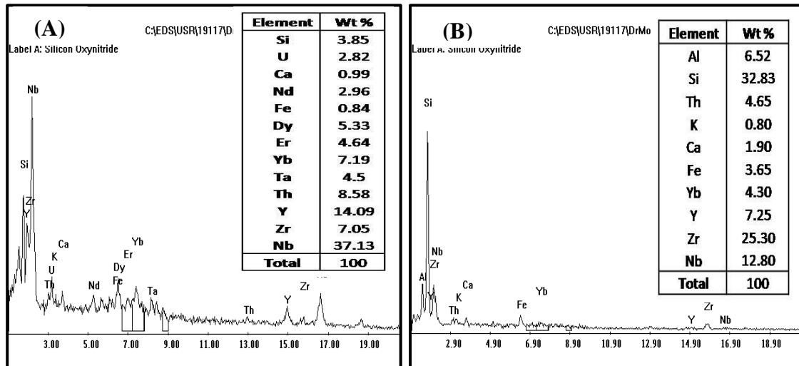
Fig. 10. EDX analysis data of float (A), sink (B) products
