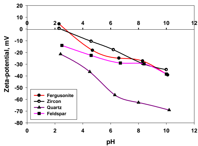
Fig. 3. Effect of pH on zeta-potential of pure fergusonite, zircon, quartz, and feldspar minerals
