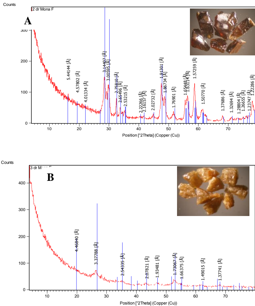
Fig. 2. X-ray diffraction patterns: (A) fergusonite (ASTM card no. 9-0443), (B) zircon (ASTM card no.01-081-0591)
