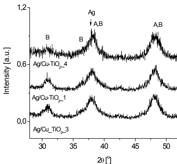
Fig. 2. XRD patterns of Ag/Cu-doped \text{TiO}_2 nanoparticles calcinated for 2 hours at 450^\circ\text{C}
