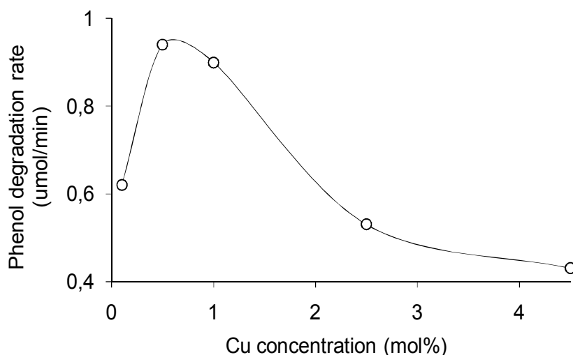
Fig. 5. Degradation rate for phenol v.s. mol% of Cu/TiO 2
