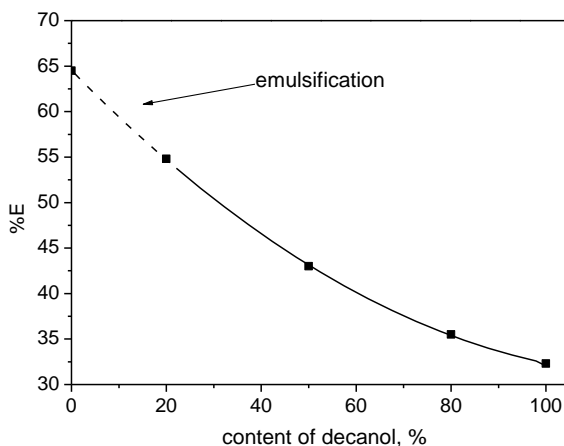
Fig. 2. Effect of n -decanol on percentage extraction of Pb(II) by R(COOH) 4 ([Pb(II)] = 5·10 -4 M, pH = 5.0; [R(COOH) 4 ] = 5·10 -4 M; contact time: 1 h)
