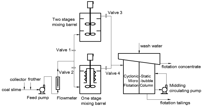
Fig.1. Equipment flow chart
