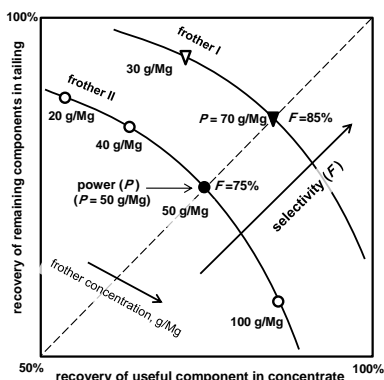
Fig. 3. Hypothetical Fuerstenau upgrading curve to show selectivity F (%) and power P (g/Mg) of flotation frothers
