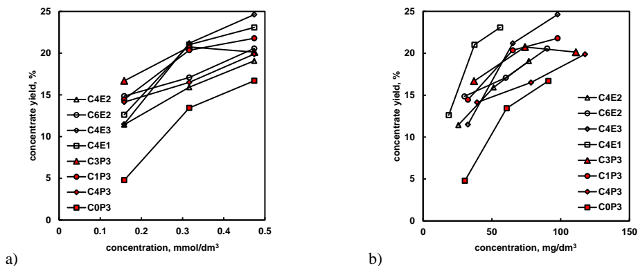
Fig. 1. Concentrate yield vs. frother dose expressed in (a) mmol/dm 3 and (b) mg/dm 3 after 16 min of flotation
