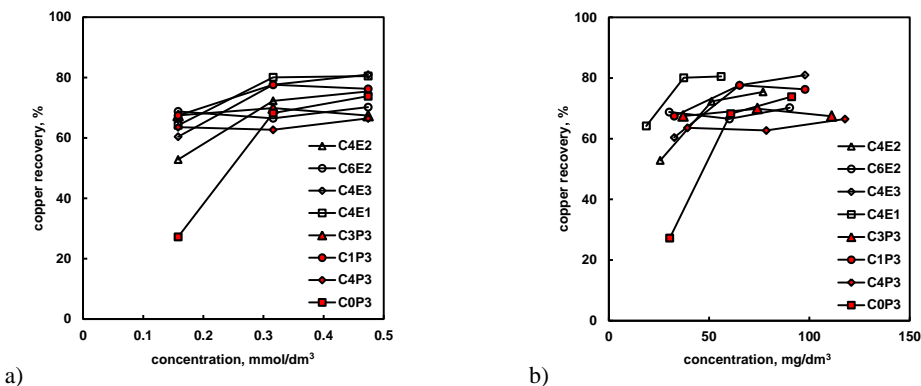
Fig. 2. Copper recovery vs. frother dose expressed in (a) mmol/dm 3 and (b) mg/dm 3 after 16 min of flotation
