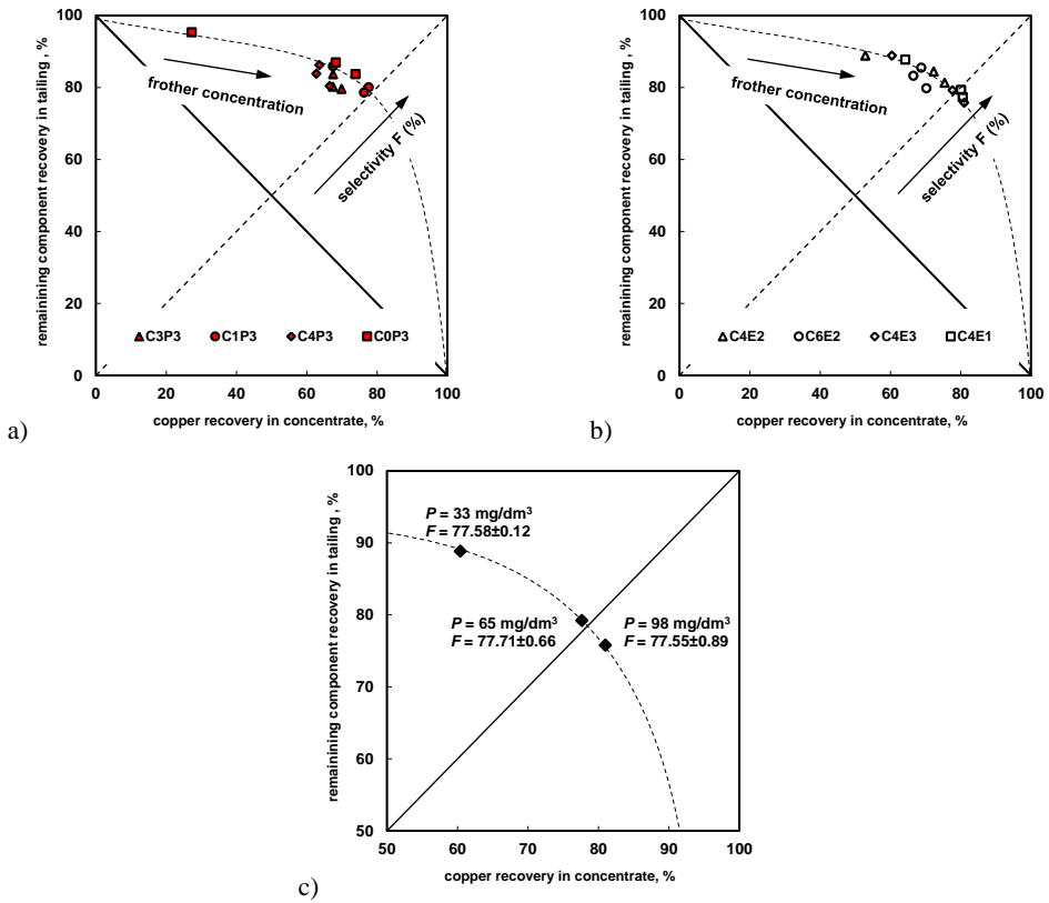
Fig. 4. Fuerstenaу upgrading curves for flotation of copper ore in the presence of (a) poly(propylene glycol) alkyl ethers, (b) poly(ethylene glycol) alkyl ethers and (c) C 4 E 3 as an example. Experimental data points were approximated with Eq. 1.
