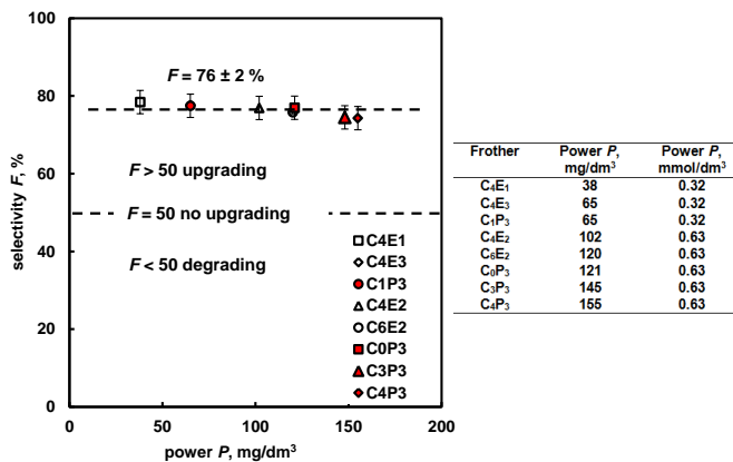
Fig. 5. Selectivity F ( 76 \pm 2\% ) and power P (in \text{mg}/\text{dm}^3 and \text{mmol}/\text{dm}^3 ) of tested frothers
