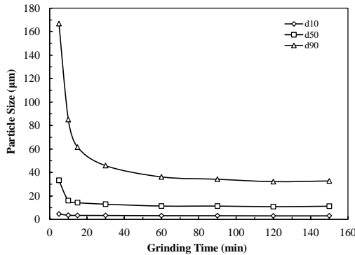
Fig. 3. Change in particle size ( d_{10} , d_{50} , and d_{90} ) with grinding time
