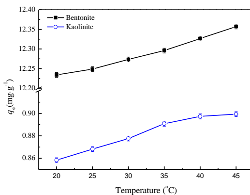
Fig. 7. Effect of system temperature on Zn(II) adsorption
