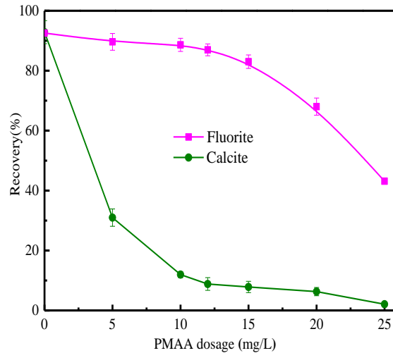
Fig. 5. The impact of PMAA dosage on the flotation of fluorite and calcite at pH 9.0 ( c(\text{NaOH}) : 1.2 \times 10^{-4} mol/L)
