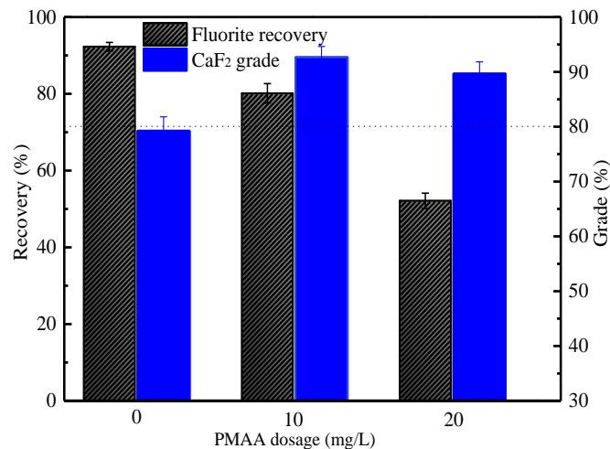
Fig. 6. Flotation results of the fluorite/calcite artificial mixture (pH=9.0, c(\text{NaOH})=1.2 \times 10^{-4} mol/L)
