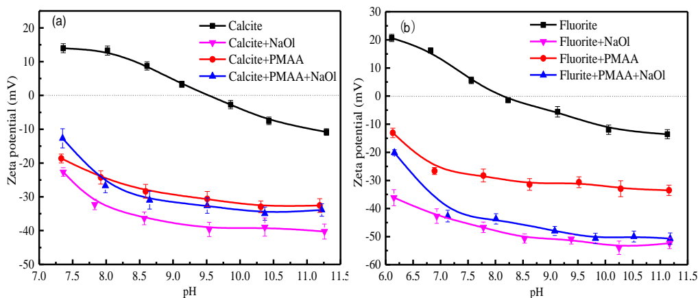
Fig. 7. The impact of pH on the zeta potentials of minerals under different condition ( c(\text{PMAA}):10 \text{ mg/L} ; c(\text{NaOl}):1.2 \times 10^{-4} \text{ mol/L} )
