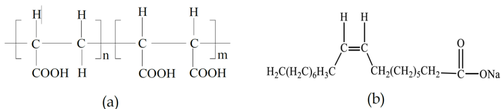
Fig. 2. The molecular structure of PMAA (a) and NaOI (b)
