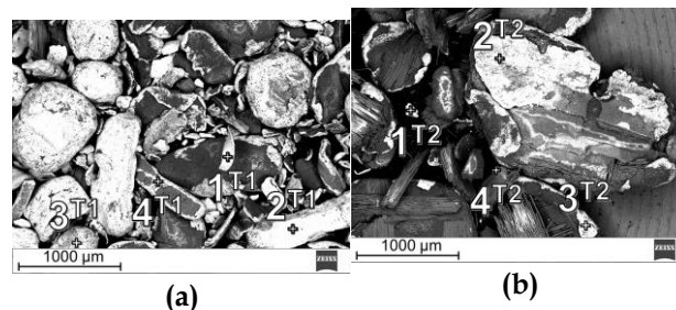
Fig. 4. The T1 and T2 products obtained from the shaking table (SEM, QBSD mode (Table 4) with marked EDS analysis points): (a) – product T1, (b) – product T2
