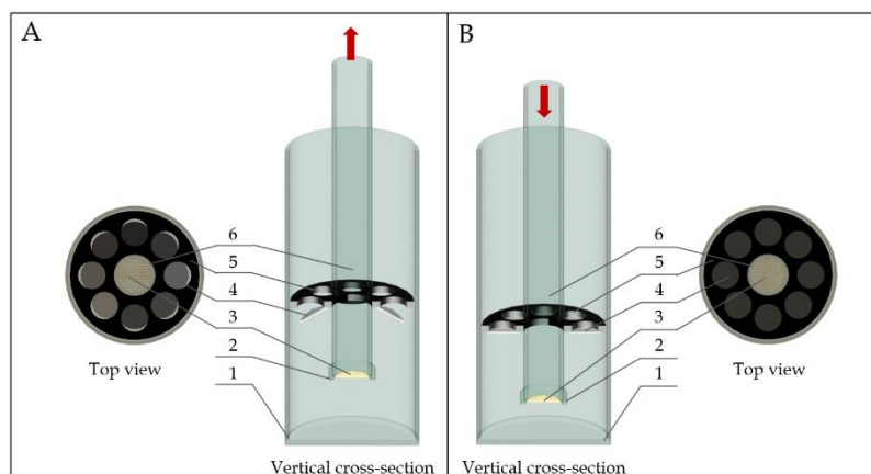
Fig. 1. Diagram of a laboratory cyclofluid separator: A – upper position, B – lower position, 1 – cylindrical tank ( \varnothing_{in} 19.5 cm), 2 – sieve clamp, 3 – sieve (mesh size 0.5 x 0.5 mm), 4 – valves, 5 – band, 6 – separation (working) chamber: \varnothing_{in} 5 cm
