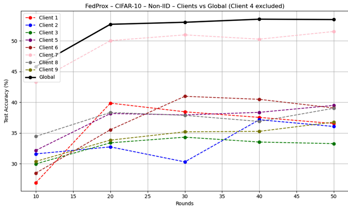
Figure 3. Client and global accuracy after removing the top-performing client
