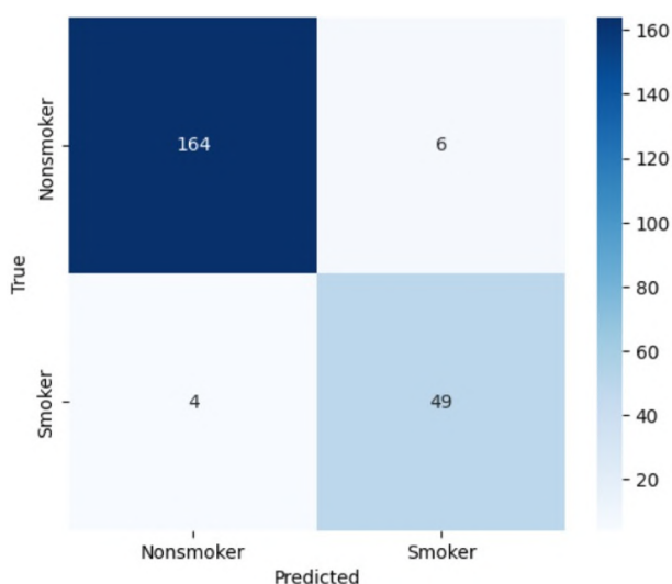
Figure 10. Confusion matrix of GNN + FT-transformer (seed 0)
