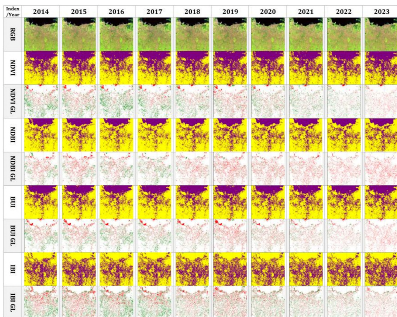
Figure 3. Annual classification and gain/loss maps for Jakarta (2014–2023). Built-up areas are shown in purple and non-built-up areas in yellow. Green indicates new urban development (gain), while red highlights areas of built-up land loss.
