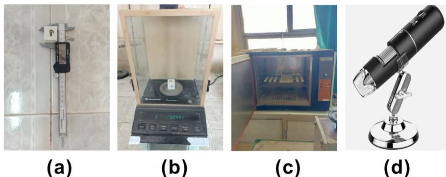
Figure 4. Testing methods for the foamed gypsum: (a) digital vernier caliper; (b) electronic balance; (c) drying oven; (d) 1000 × WiFi digital microscope
