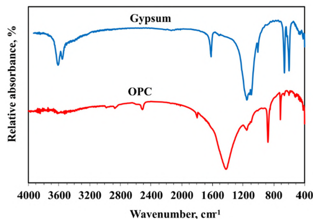
Figure 6. FTIR spectra of gypsum plaster and OPC
