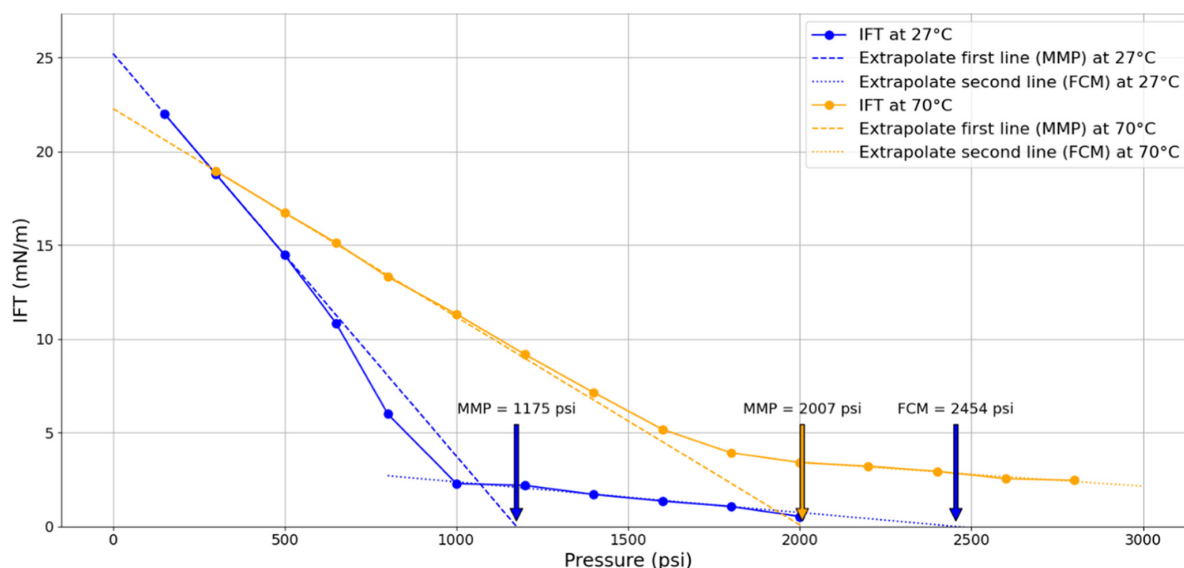
Figure 7. Measured IFT at various pressures at 27^\circ\text{C} and 70^\circ\text{C}
