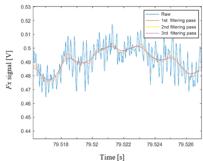
Figure 2. Results of Savitzky-Golay filtering on an example cutting force signal
