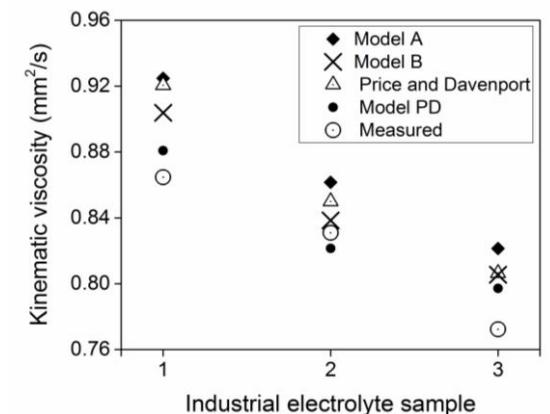
Fig. 5. Kinematic viscosity values of the industrial electrorefining electrolyte samples 1-3 measured at 65 °C vs. values modeled with the Model A, the model of Price and Davenport (1981), the Model B and the Model PD
