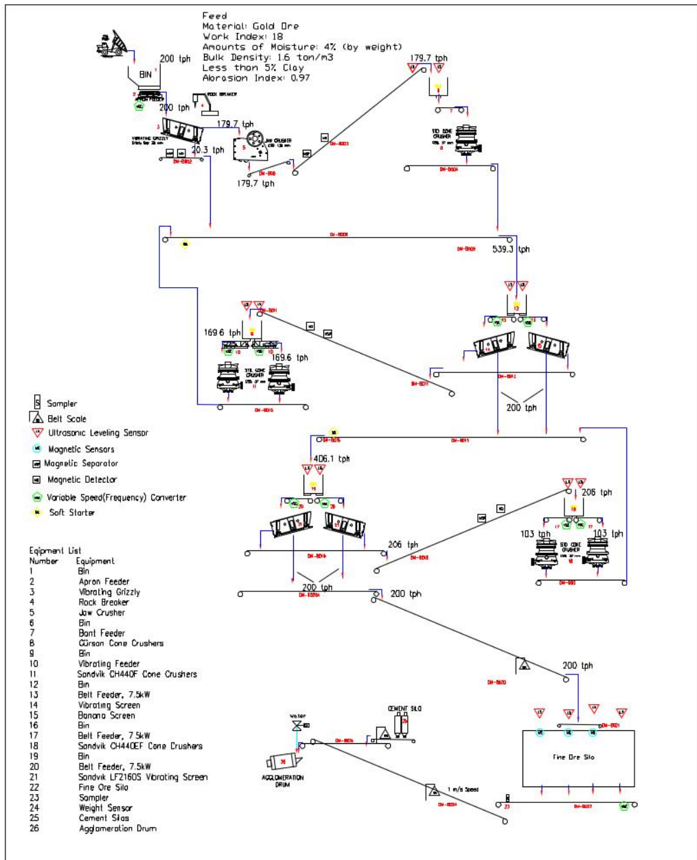
Fig. 8. Flowsheet developed after re-design
